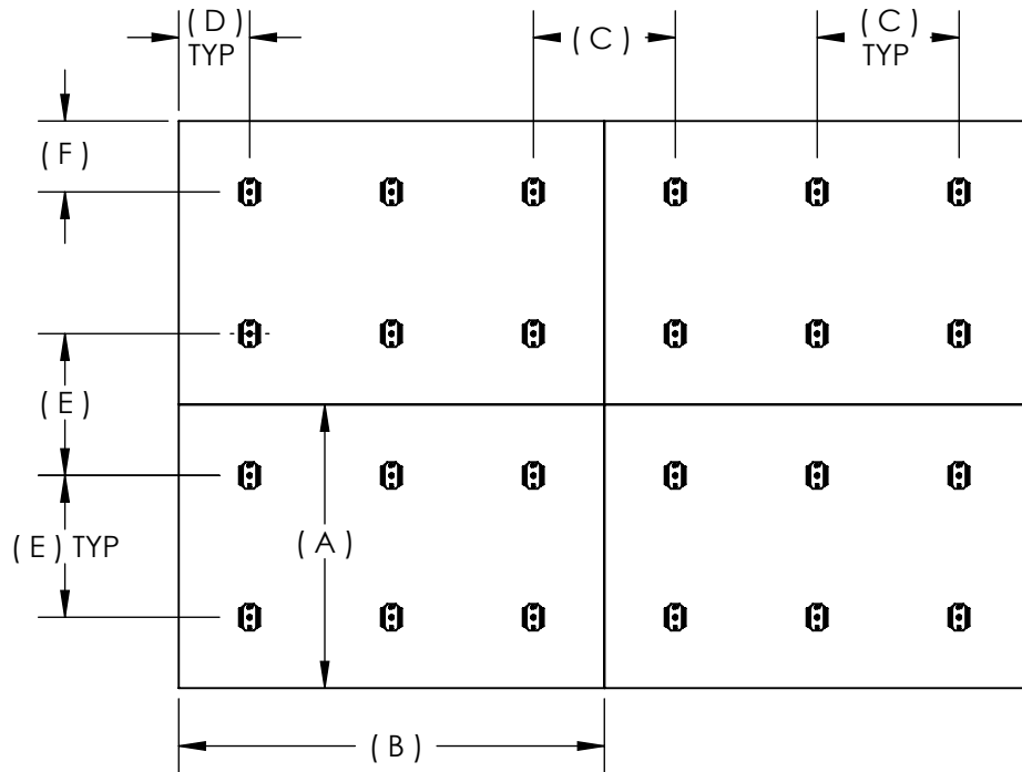
WALLS BOARD ANCHORING
