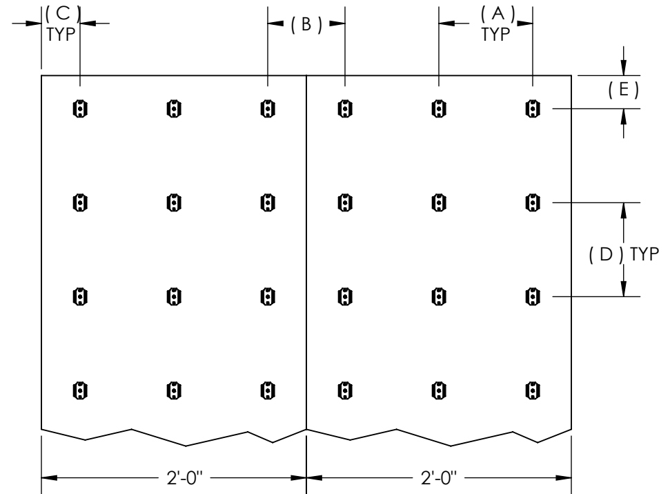
ROOF 24" WIDE BLANKET BUTT JOINTS
