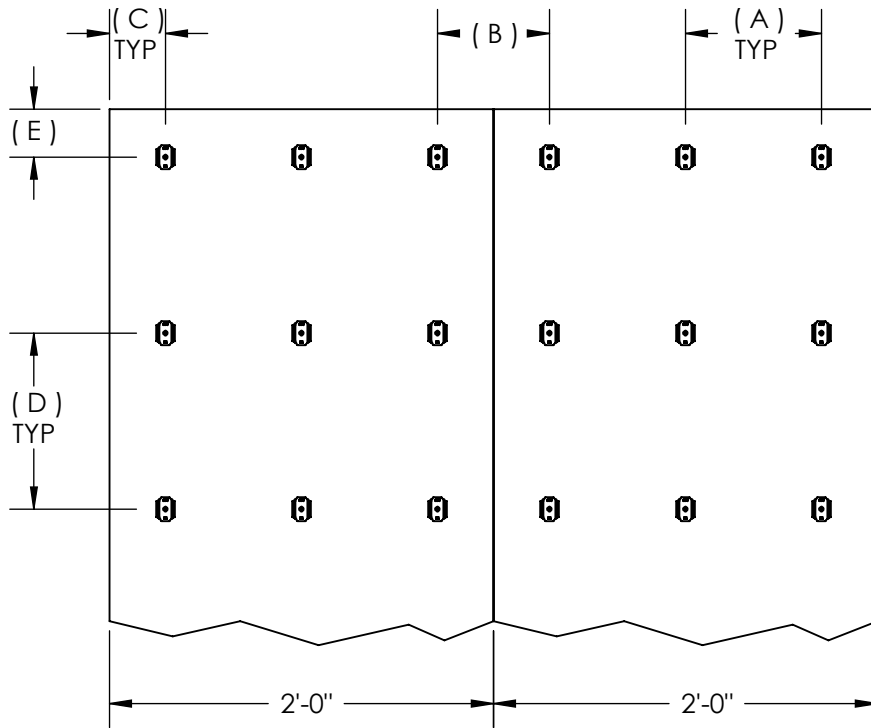
WALLS 24" WIDE BLANKET BUTT JOINTS
