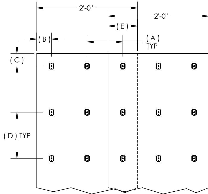
WALLS 24" WIDE BLANKET OVERLAPPED JOINTS
