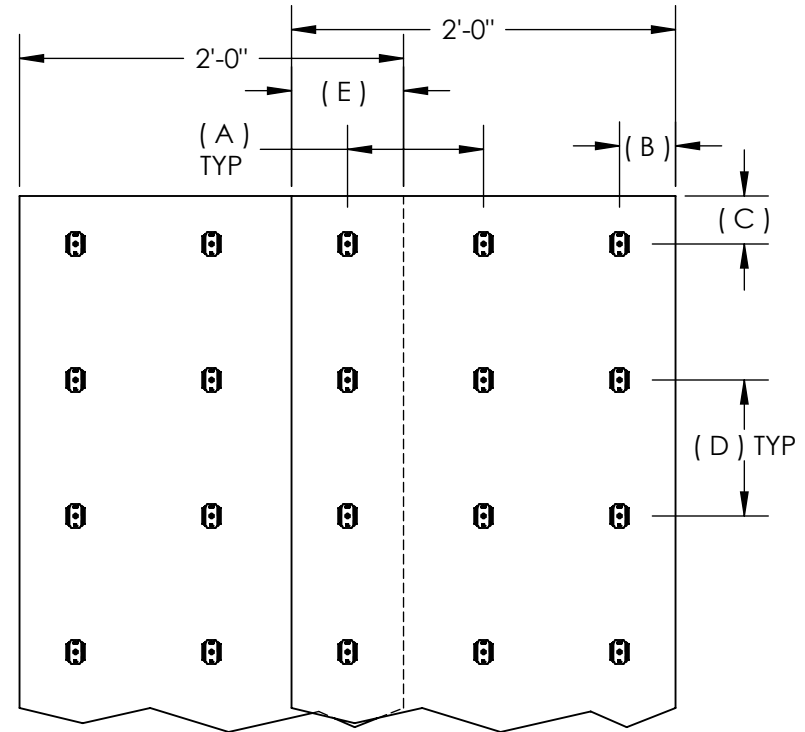
ROOF 24" WIDE BLANKET OVERLAPPED JOINTS
